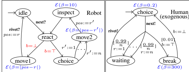
Figure 2: Illustration of automata-network encoding for the riveting application, with robot workflow of type (3b), and human workflow of type (1b) and (2a). \mathcal{E}(\beta=x) denotes the exponential distribution with mean x .
